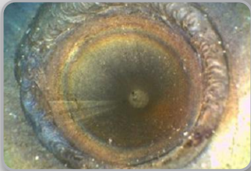
Orbital Weld
